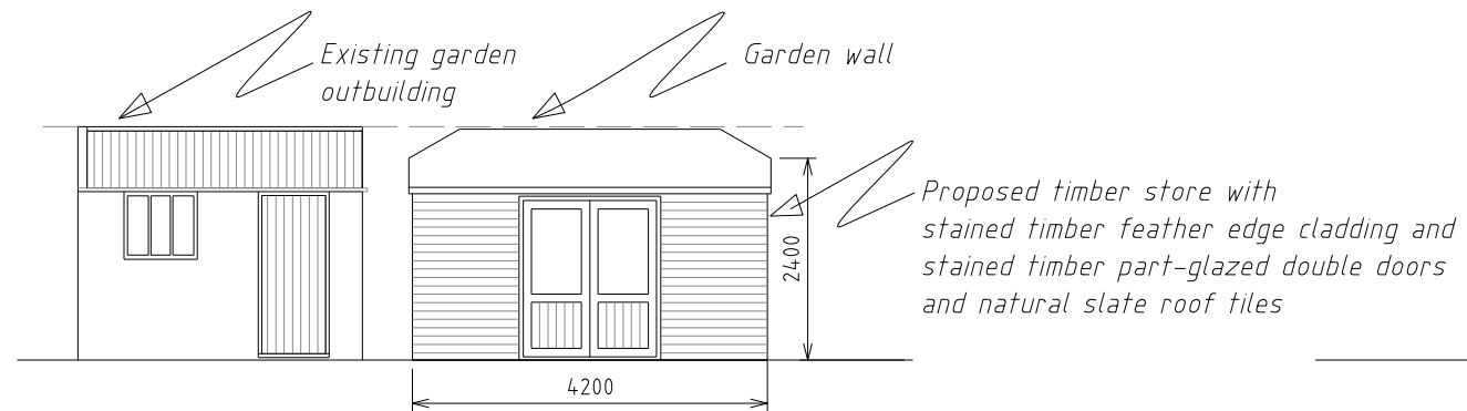
FRONT ELEVATION
