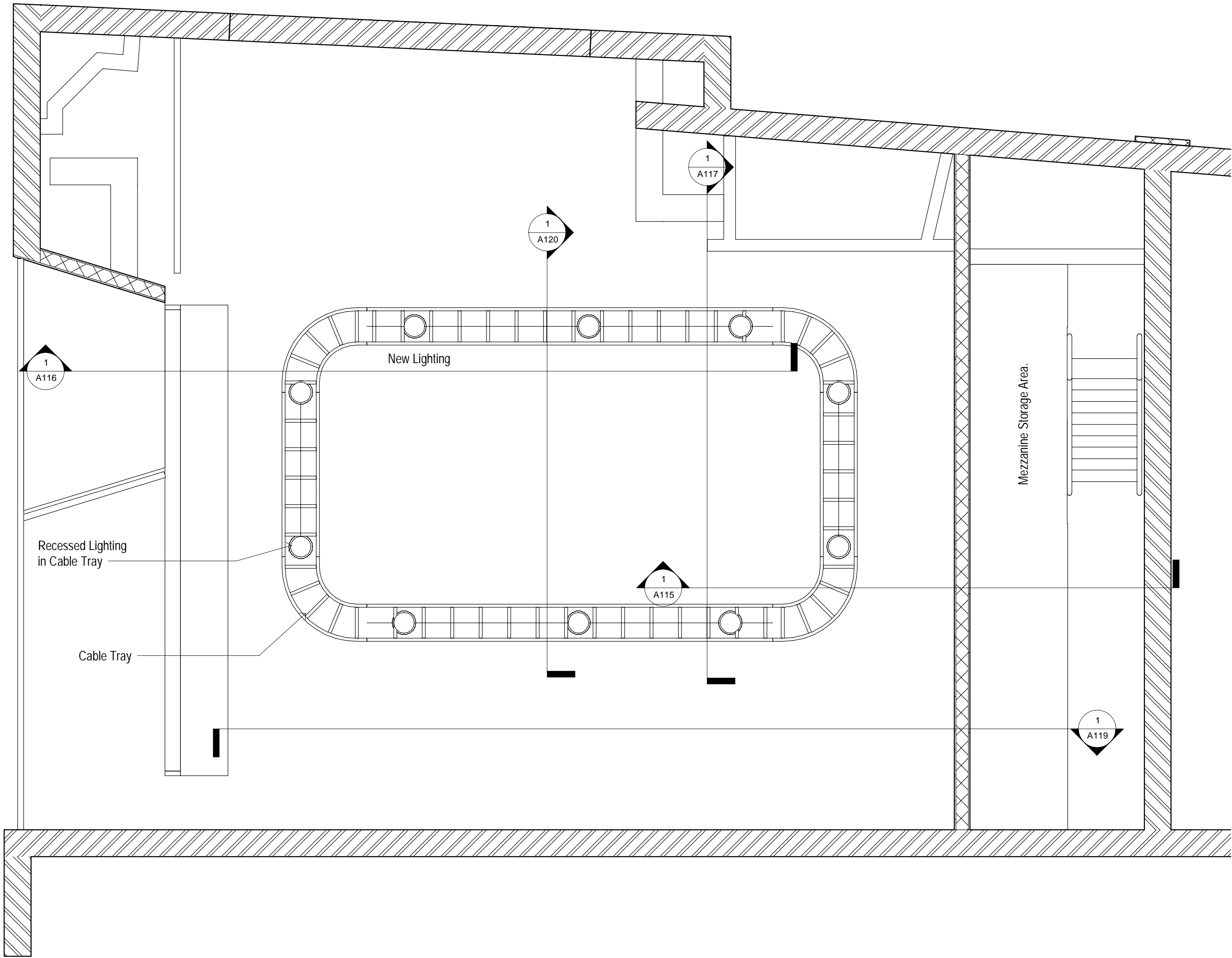
1 B-Proposed Mezzanine Storage 1 : 25
