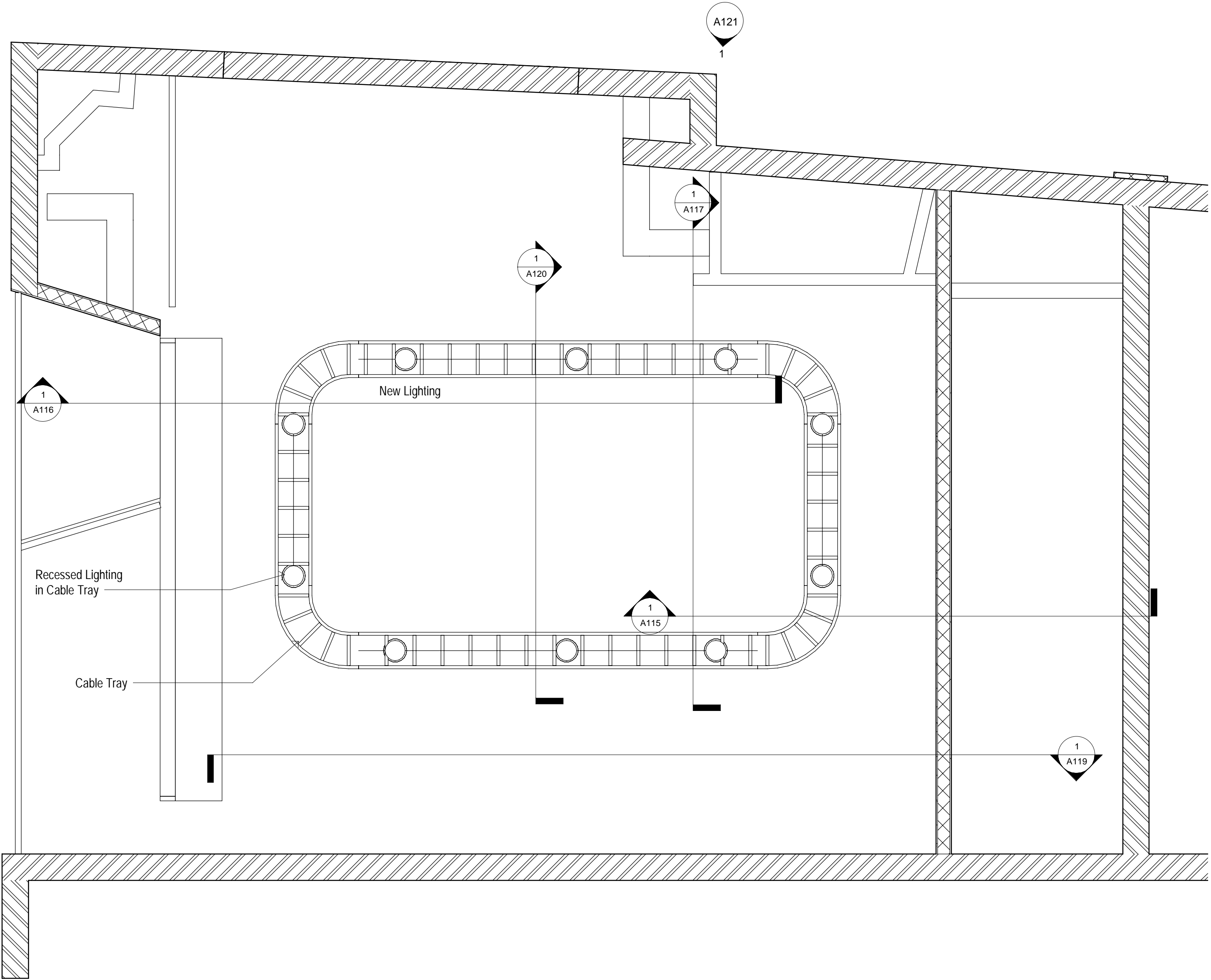
1 B-Proposed Mezzanine Storage 1 : 25
