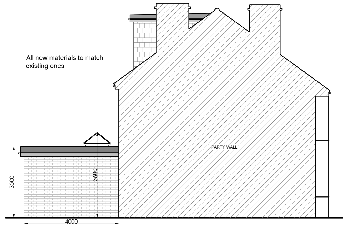
PROPOSED OPPOSITE SIDE ELEVATION
