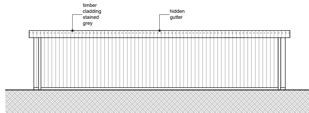
6 PROPOSED FRONT ELEVATION
