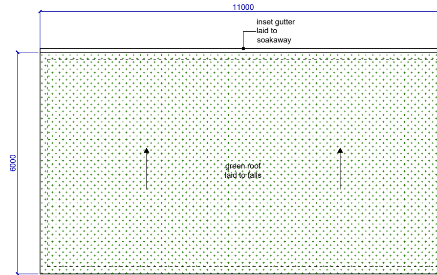
2 PROPOSED ROOF PLAN
