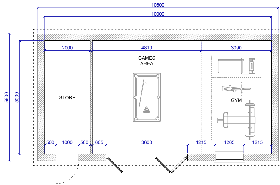
1 PROPOSED FLOOR PLAN
