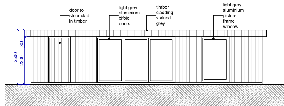
4 PROPOSED FRONT ELEVATION
