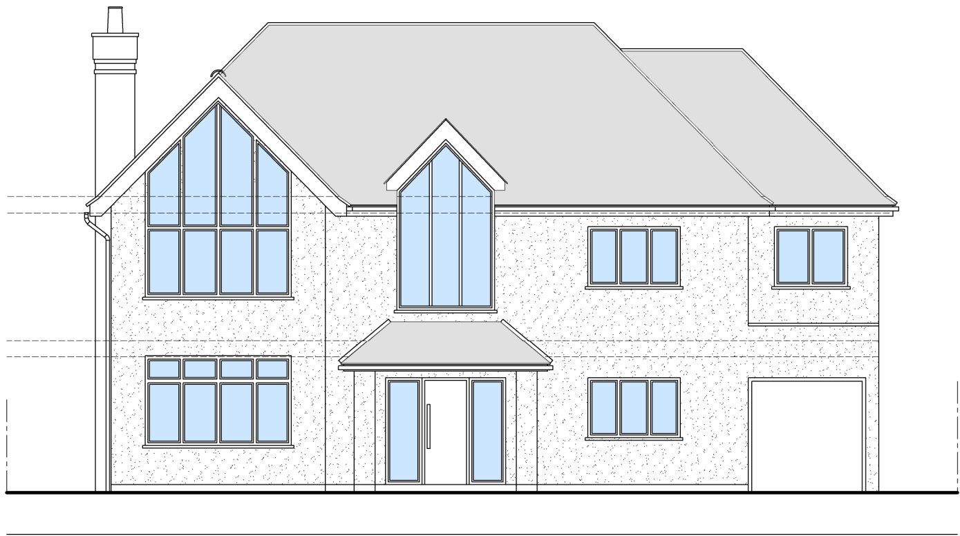
EXISTING DWELLING FRONT ELEVATION
