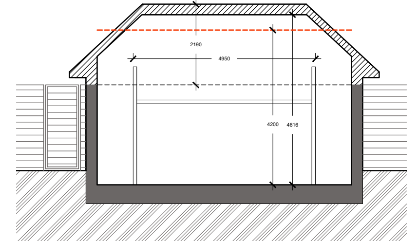
PROPOSED SECTION
