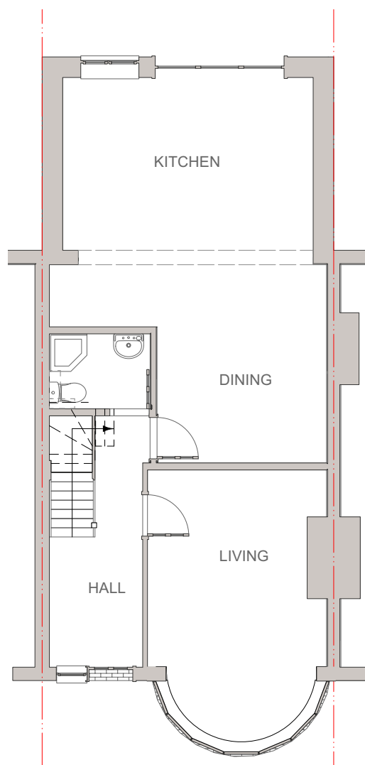
01 GROUND FLOOR PLAN Scale: 1:100 0 1 2 3 4 5 M
