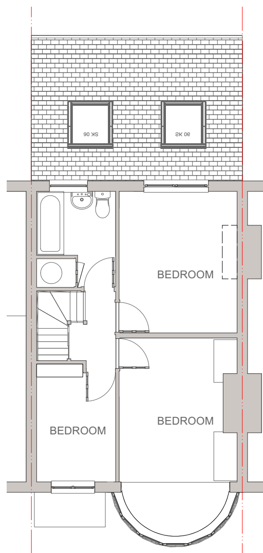
02 FIRST FLOOR PLAN Scale: 1:100
