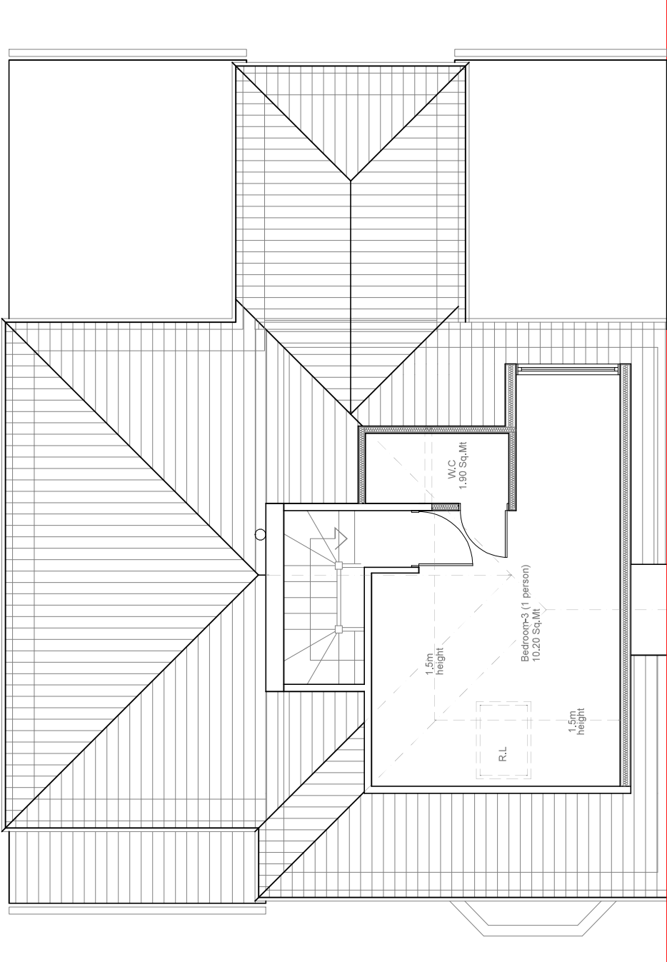
PROPOSED LOFT PLAN 1:50
