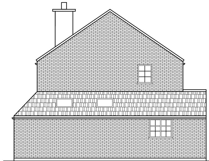
PROPOSED SIDE ELEVATION-01
