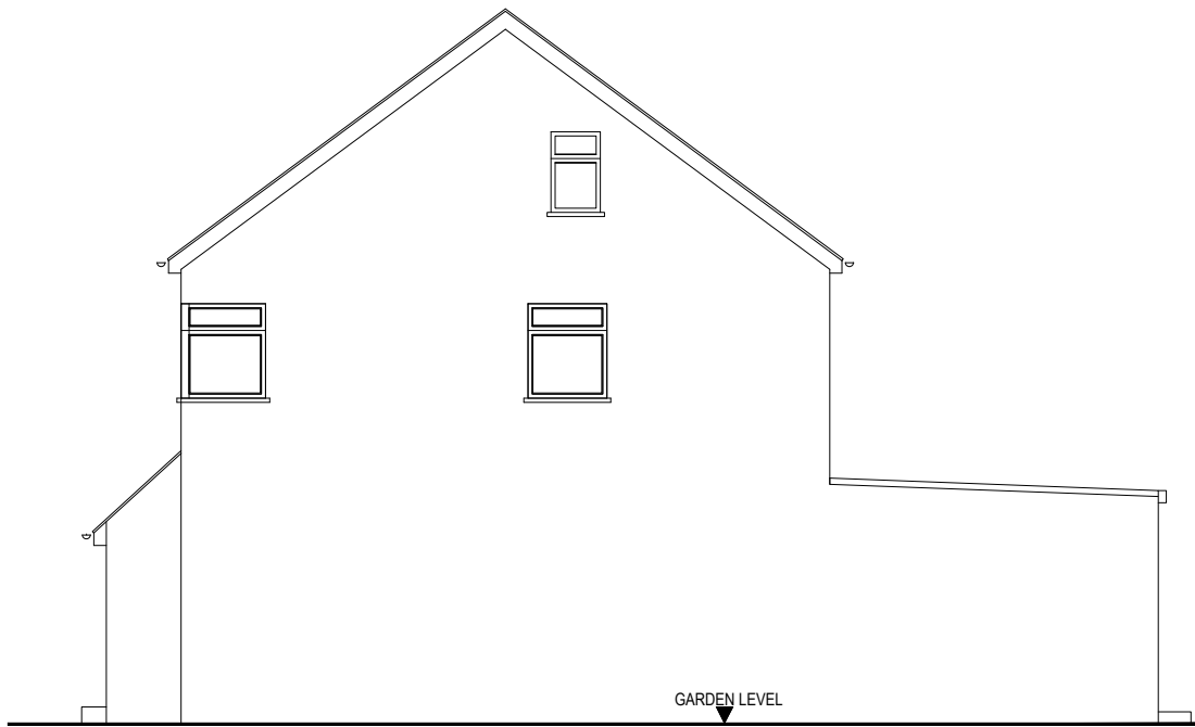
EXISTING SIDE ELEVATIONS
