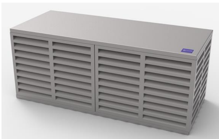
Figure 5.5 – Louvre Enclosure – 12dB reduction Calculations can be seen in Appendix B.
