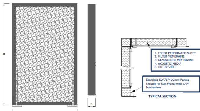
Figure 5.5.1 – Sample Acoustic screen
