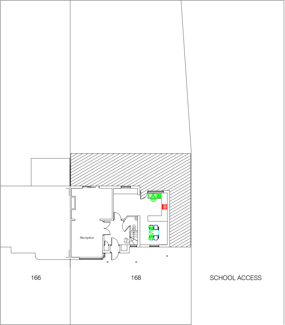
PROPOSED BLOCK PLAN SCALE 1:200
