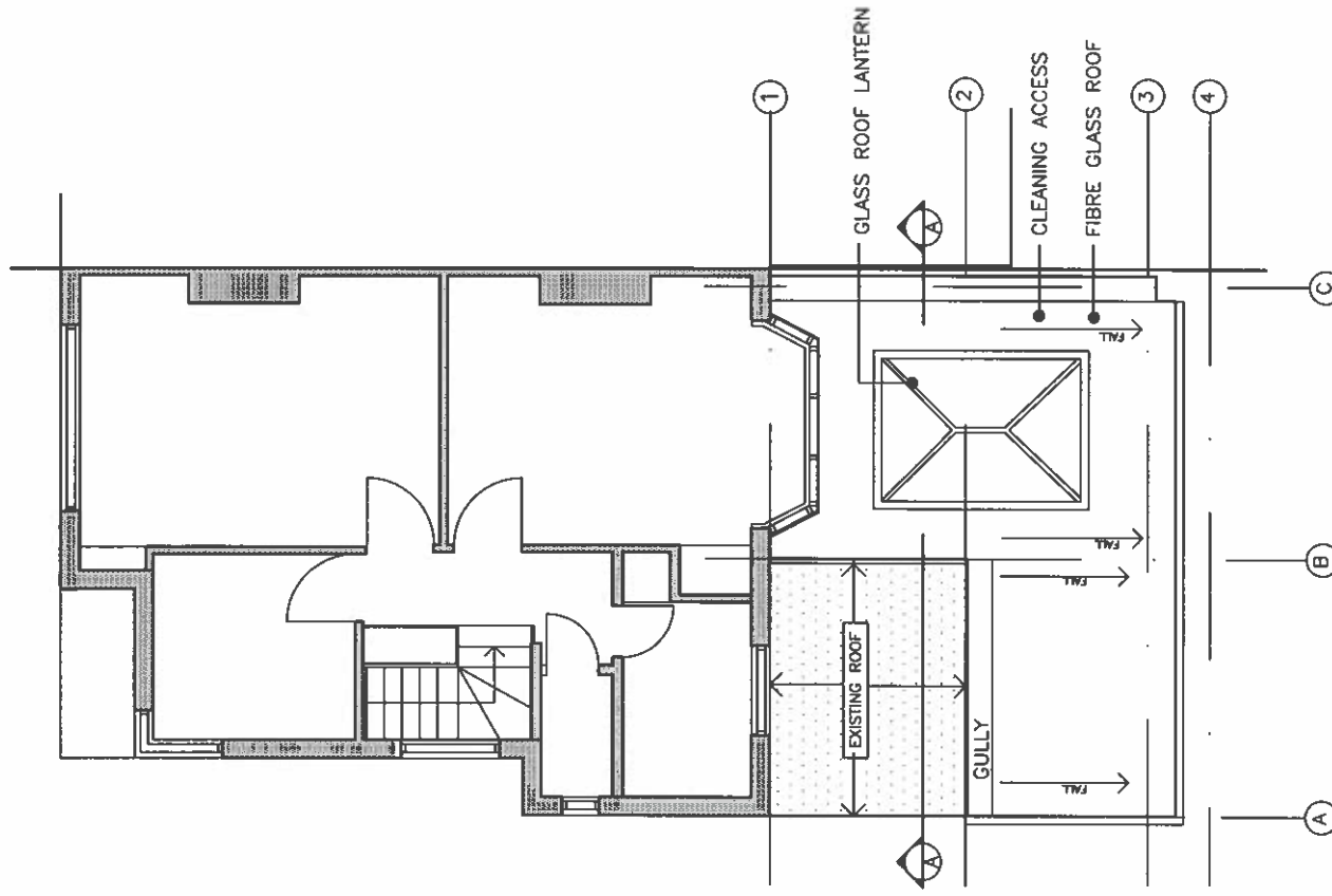
PROPOSED NEW ROOF PLAN @ FIRST FLOOR
