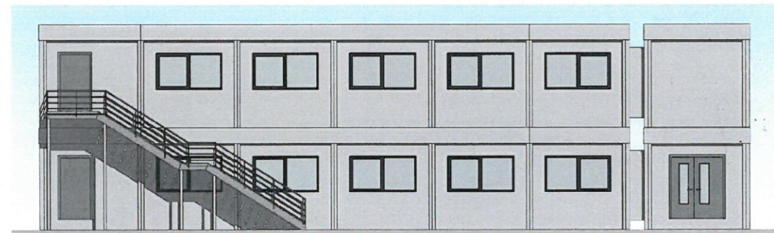
5 South Elevation 1 : 125
