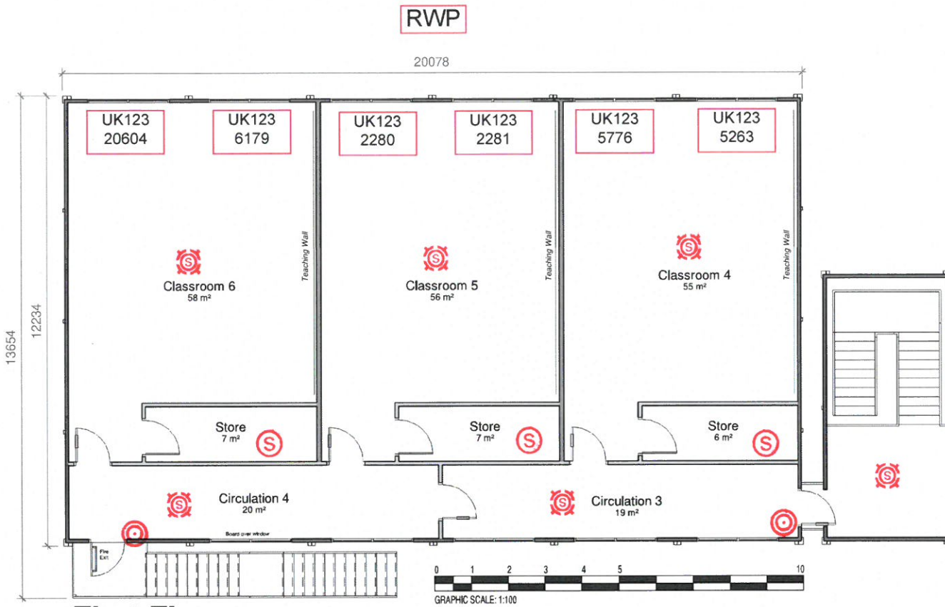
2 First Floor 1 : 100
