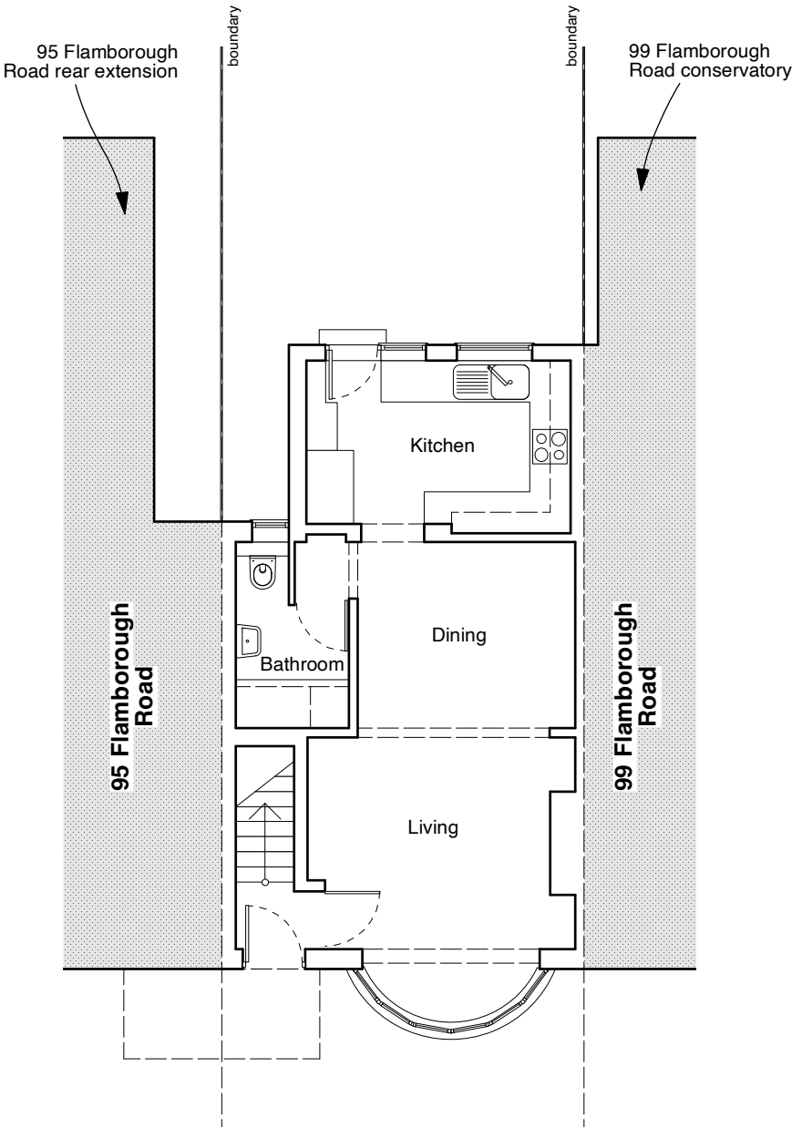
Ground Floor
