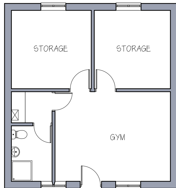
1:100 FLOOR PLAN
