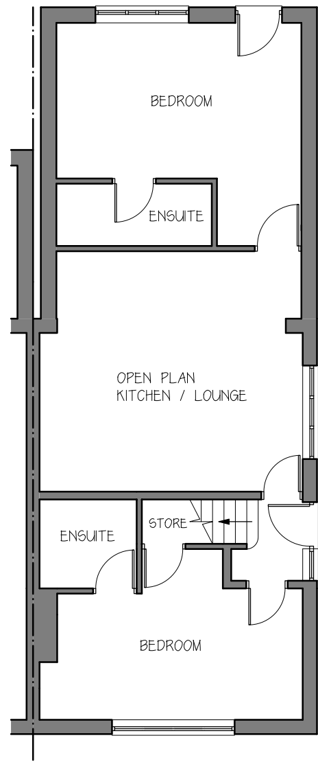
PROPOSED GROUND FLOOR PLAN (unchanged)
