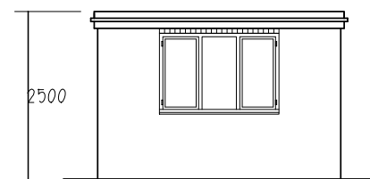
1:100 FRONT ELEVATION
