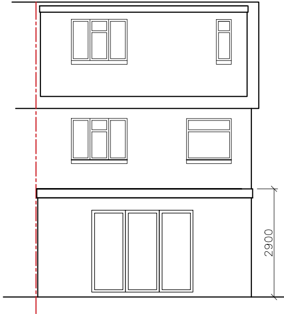
PROPOSED REAR ELEVATION PLAN SCALE= 1:100
