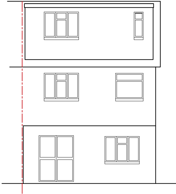
EXISTING REAR ELEVATION PLAN SCALE= 1:100
