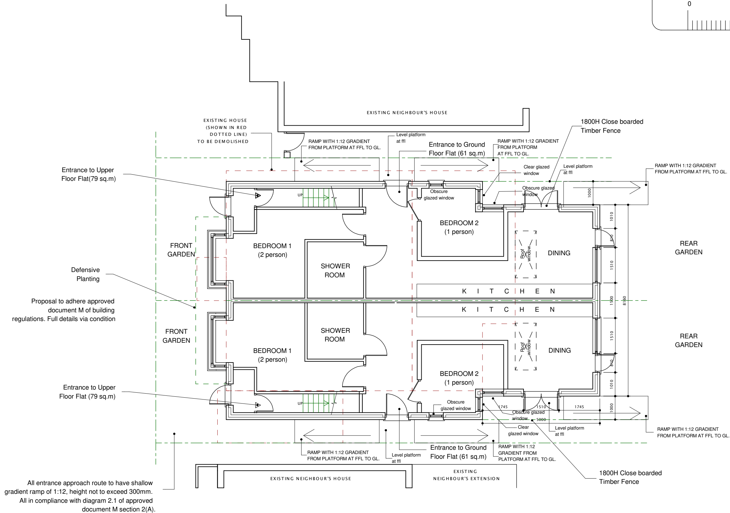
PROPOSED GROUND FLOOR PLAN ( GROUND FLOOR FLATS- 2 BEDROOMS, 3 PERSON WITH MIN. 61 SQ.M GIA)
