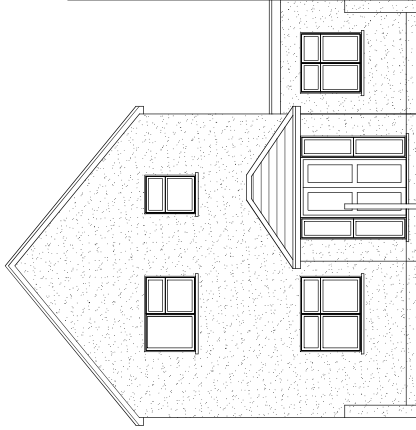
Existing Front Elevation Scale 1:100
