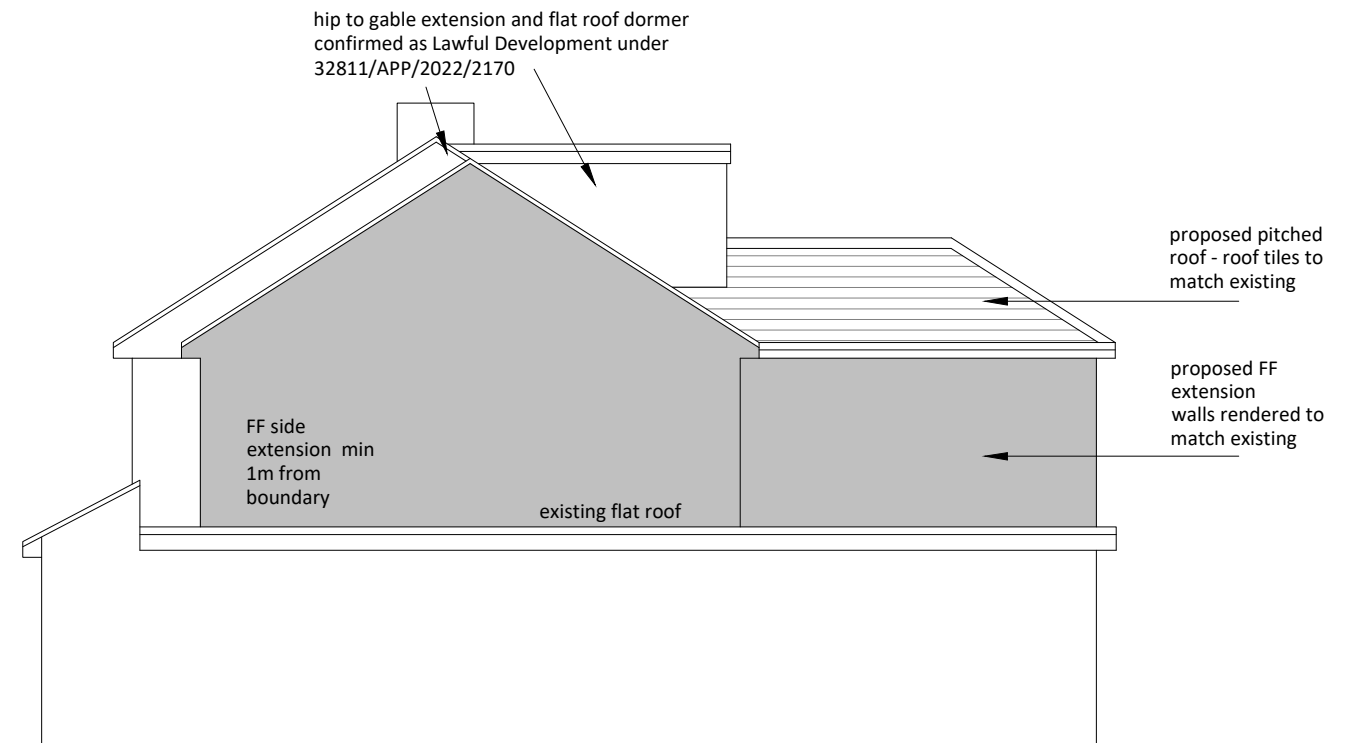
SIDE ELEVATION (NORTH-WEST) - PROPOSED
