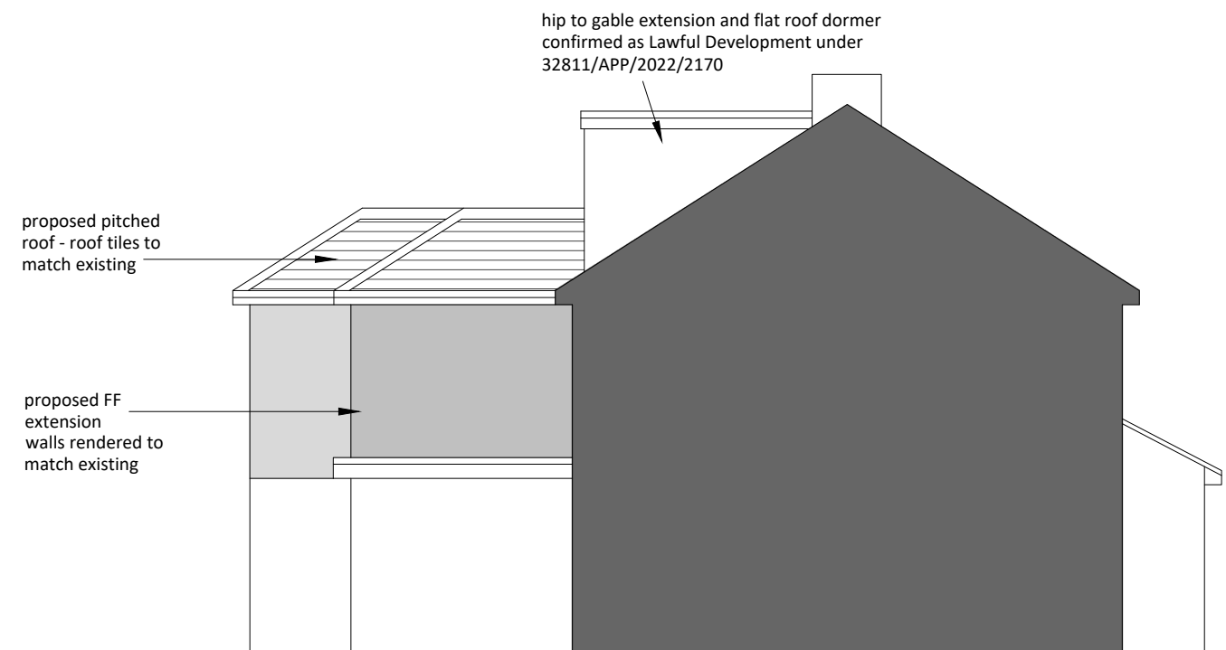
SIDE ELEVATION (SOUTH-EAST) - PROPOSED
