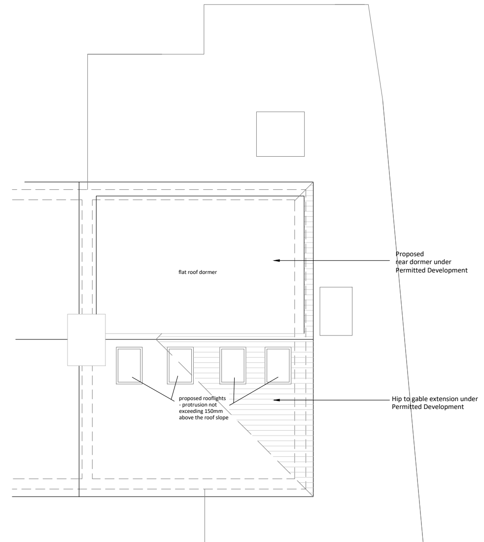
ROOF - PROPOSED
