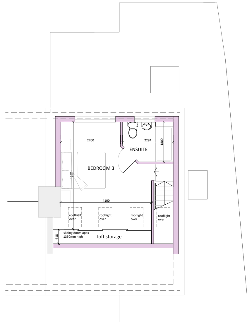
SECOND FLOOR - PROPOSED
