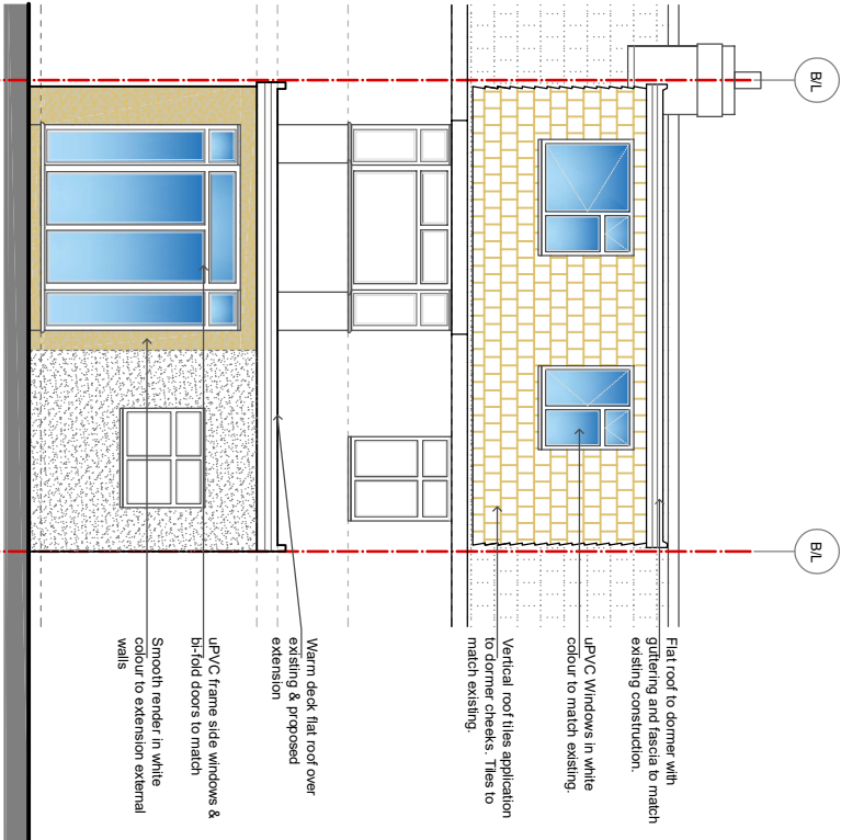
REAR ELEVATION AS PROPOSED
