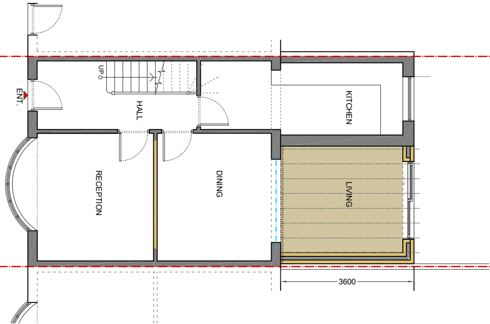
GROUND FLOOR PLAN AS PROPOSED 5 CEDAR AVENUE, HAYES - UB3 2NE
