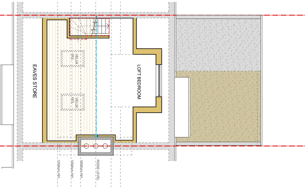
LOFT PLAN AS PROPOSED 5 CEDAR AVENUE, HAYES - UB3 2NE
