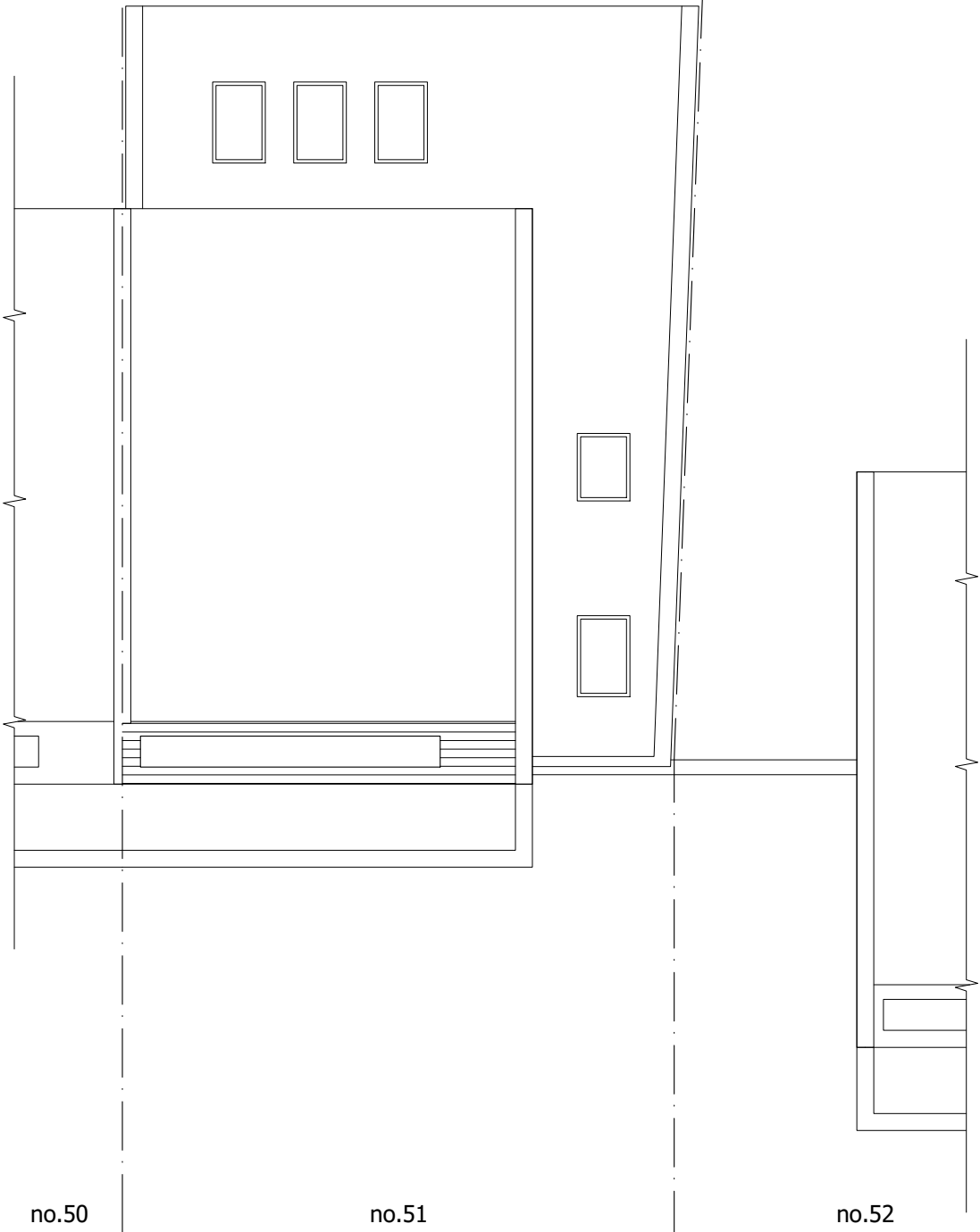
roof plan
