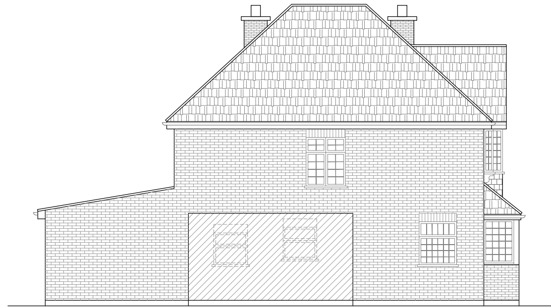
EXISTING SIDE ELEVATION-2
