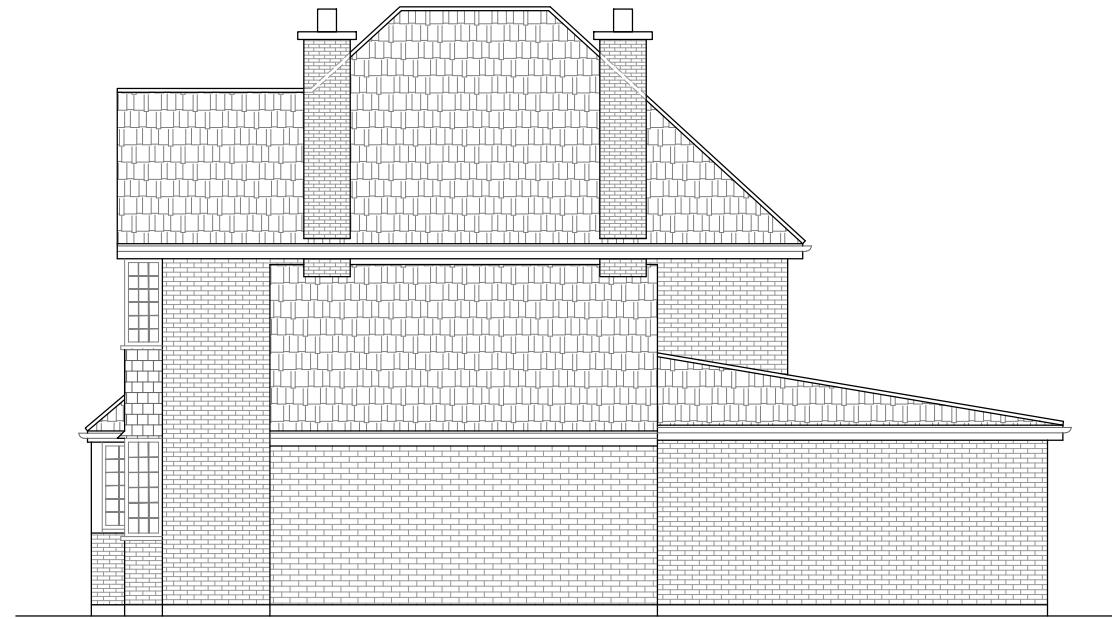
EXISTING SIDE ELEVATION-1
