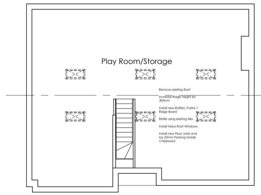
Proposed Loft Plan
