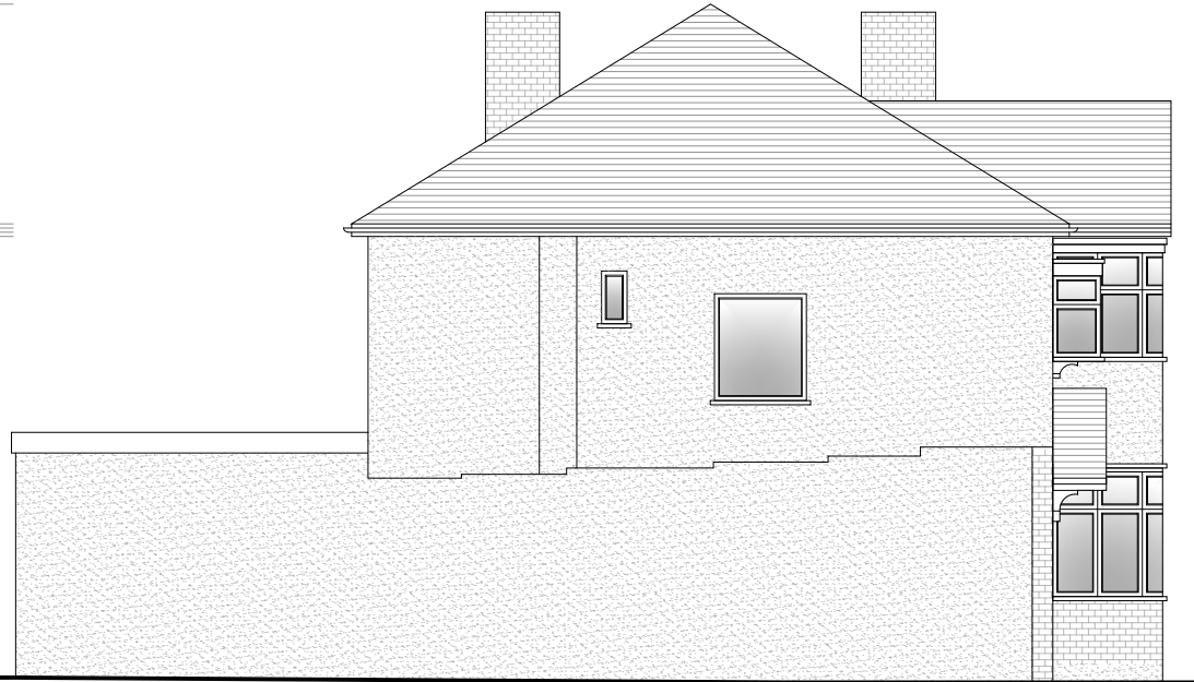
9 Existing Side Elevation Scale 1/100
