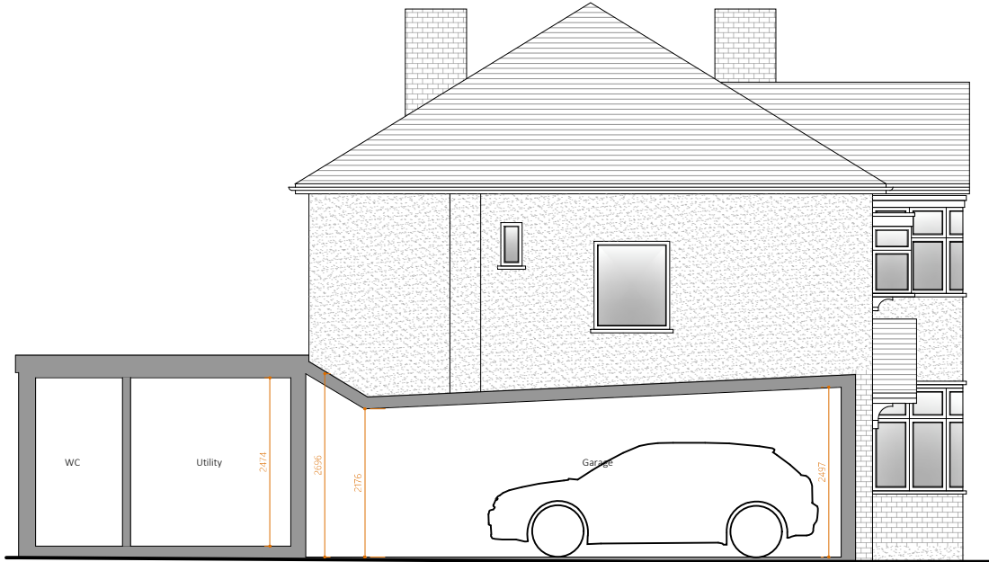
8 Existing Side Section Scale 1/100
