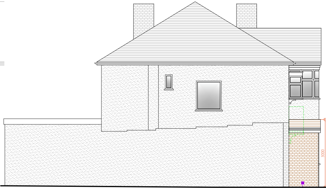
9 Proposed Side Elevation
