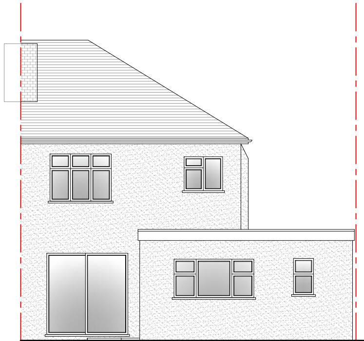
6 Proposed Rear Elevation
