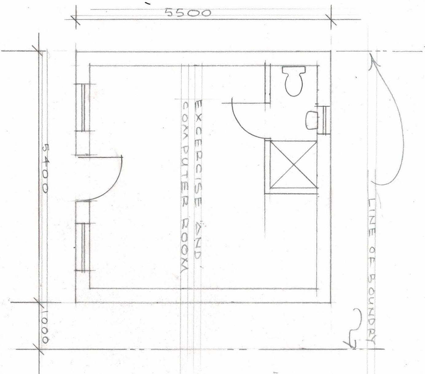
PLAN
