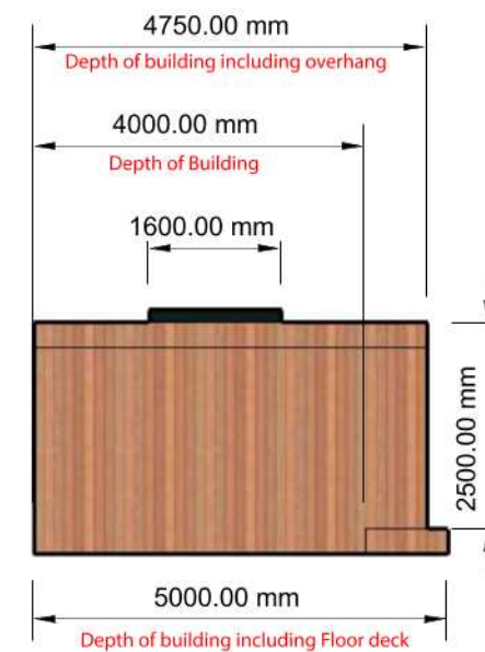
East Elevation
