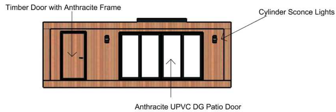
South Elevation
