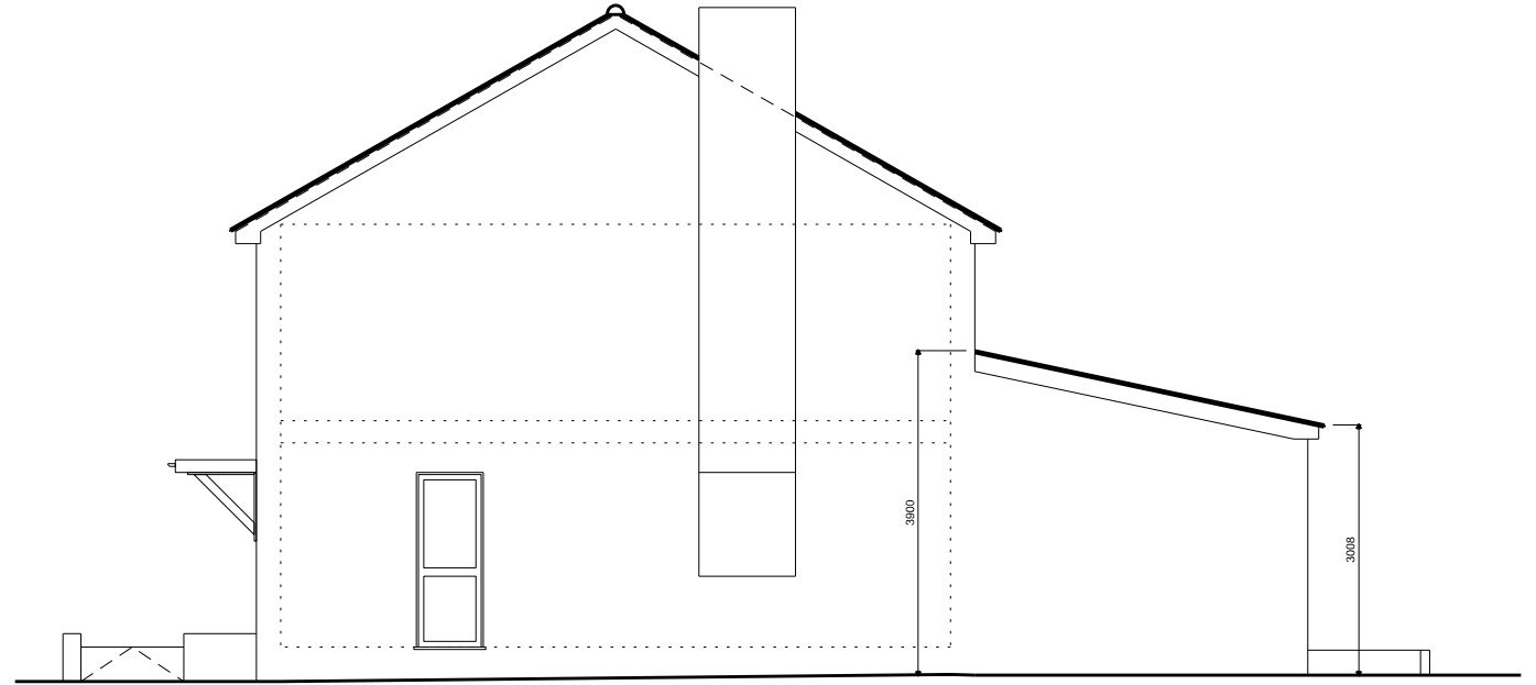
02 Proposed Side Elevation (North)
