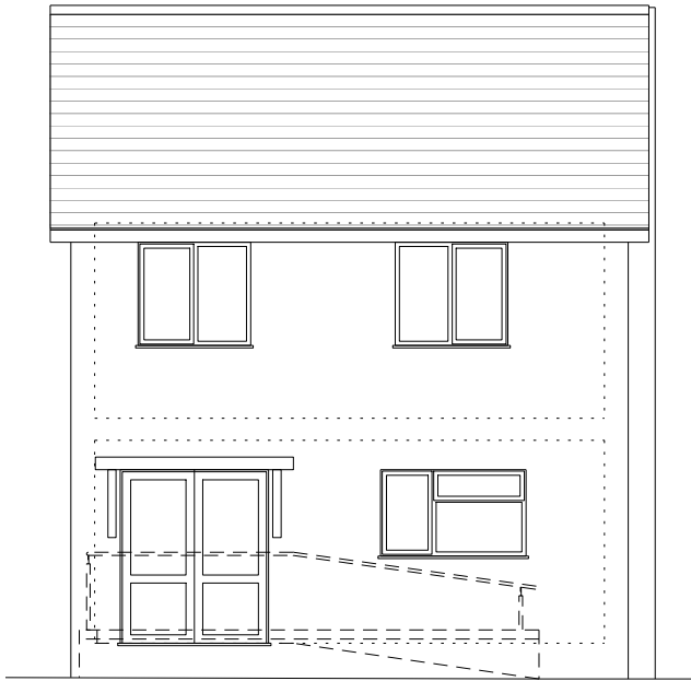
01 Proposed Front Elevation (East)
