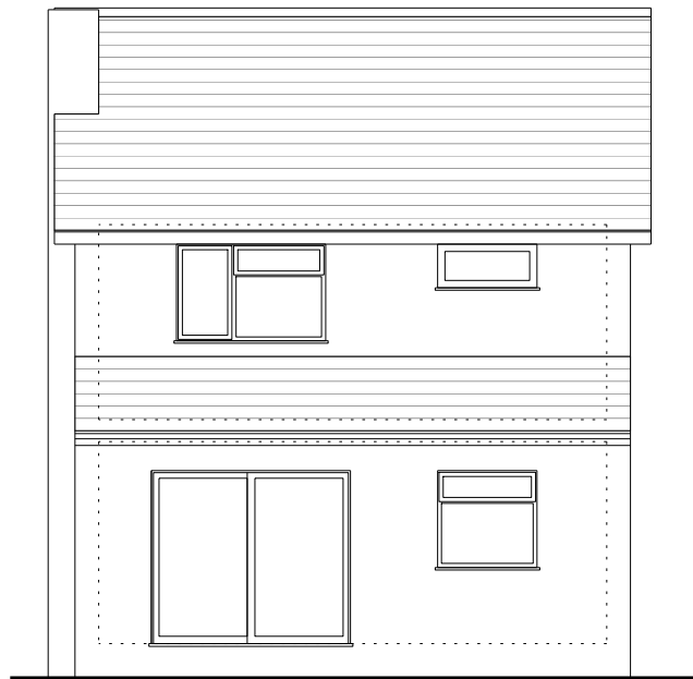
03 Proposed Rear Elevation (West)
