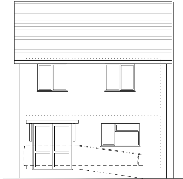
01 Proposed Front Elevation (East)
