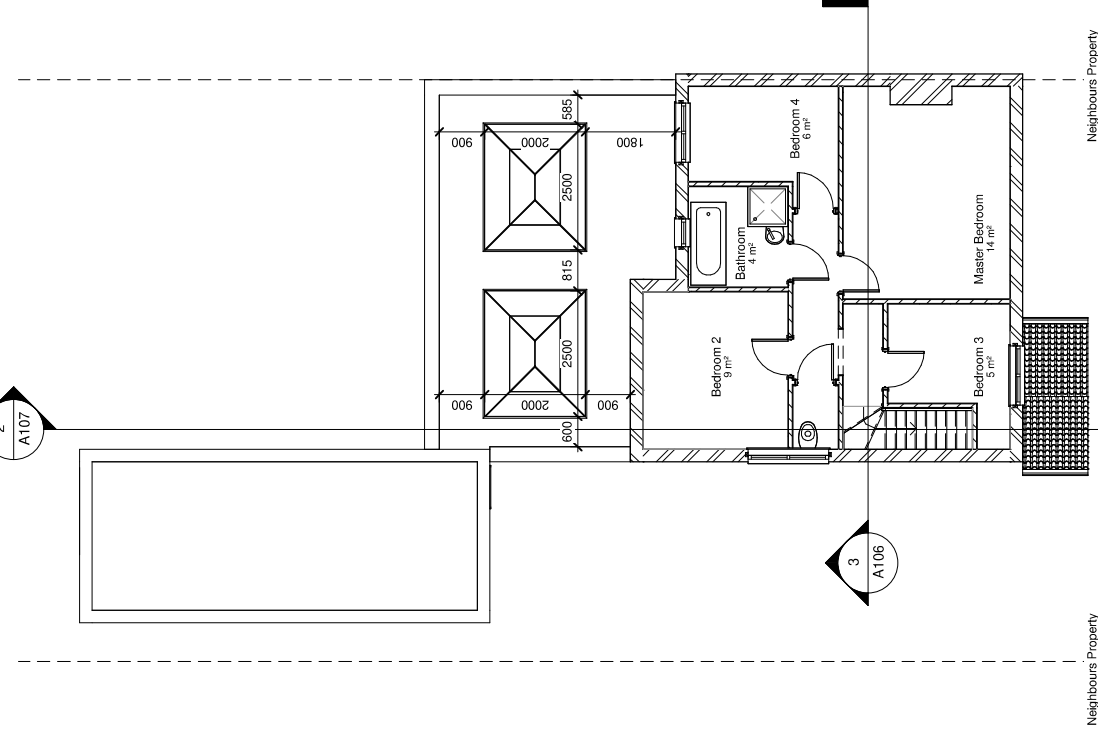
2 01- Proposed 1 : 100
