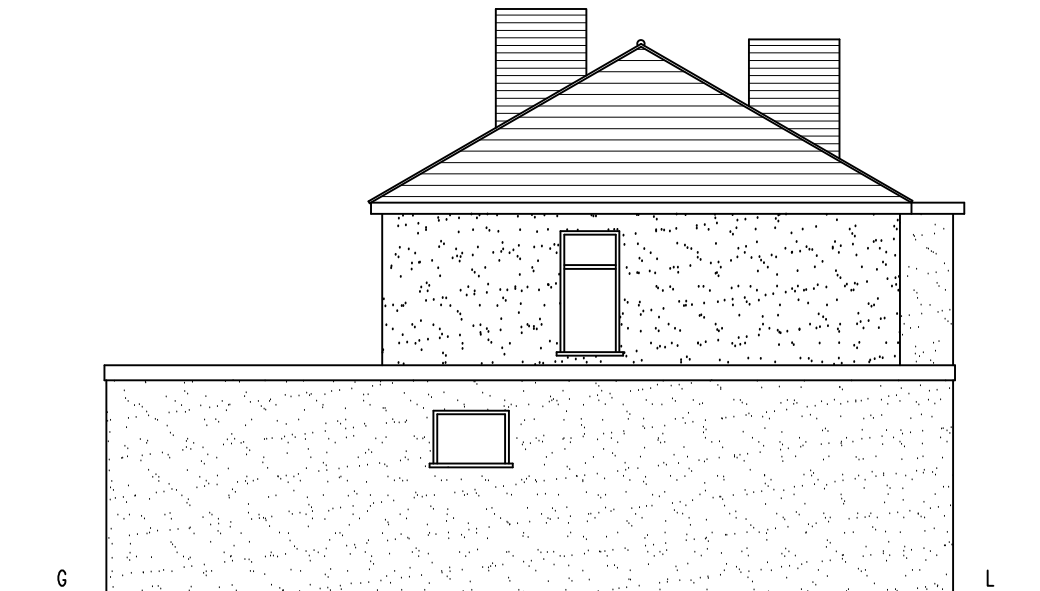
EXISTING SIDE (NORTH) ELEVATION
