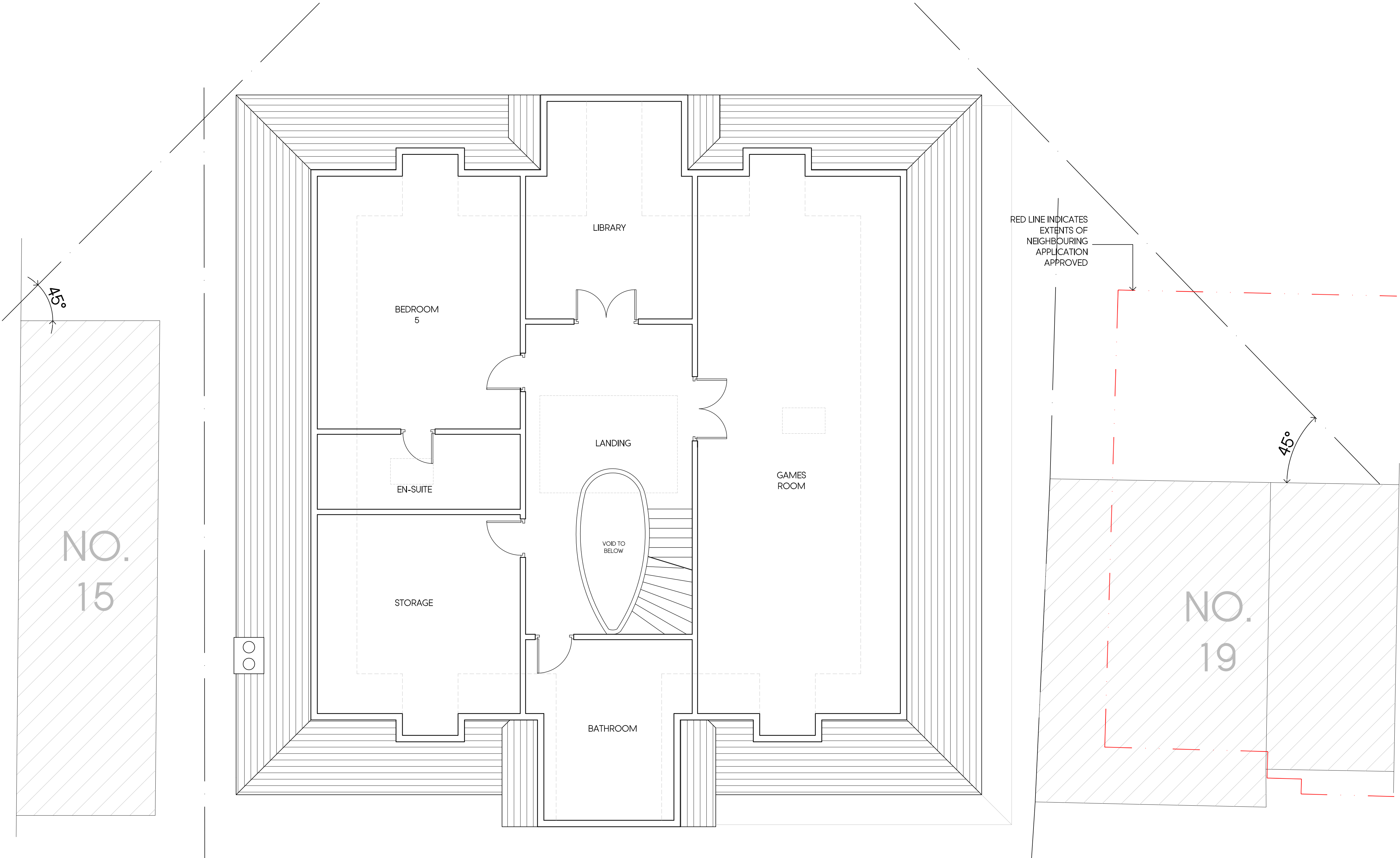
PROPOSED LOFT PLAN
