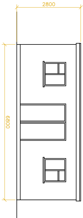
EXISTING FRONT ELEVATION
