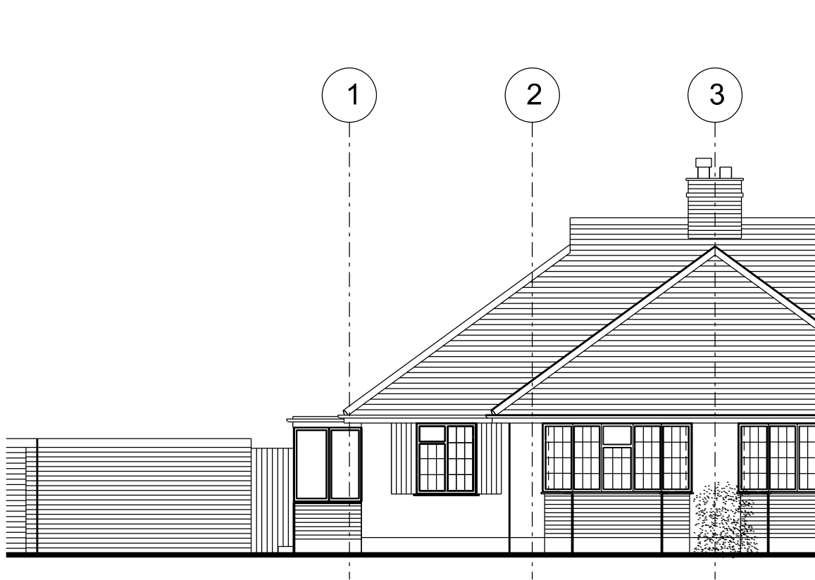
01 EXISTING FRONT ELEVATION
