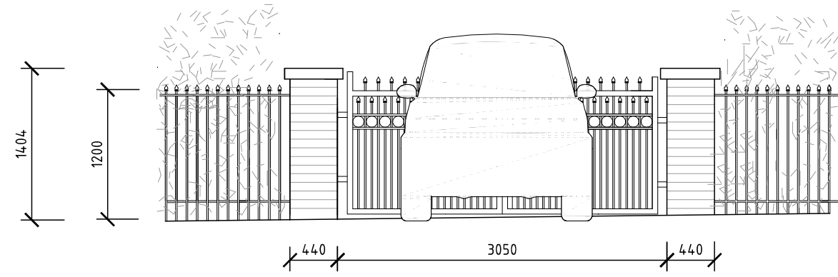
TYPICAL GATE DETAIL SCALE 1 : 50
