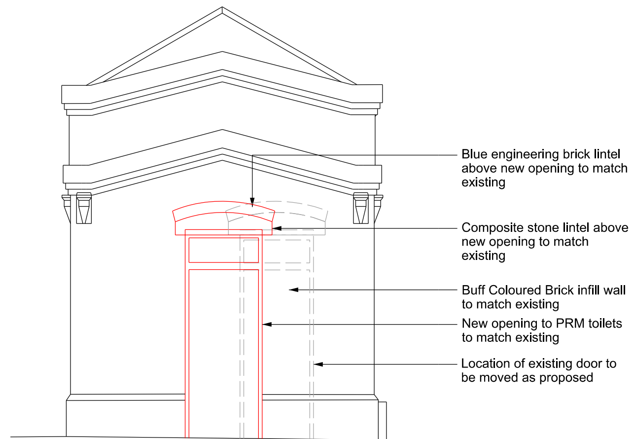
2 EAST ELEVATION 1:50
