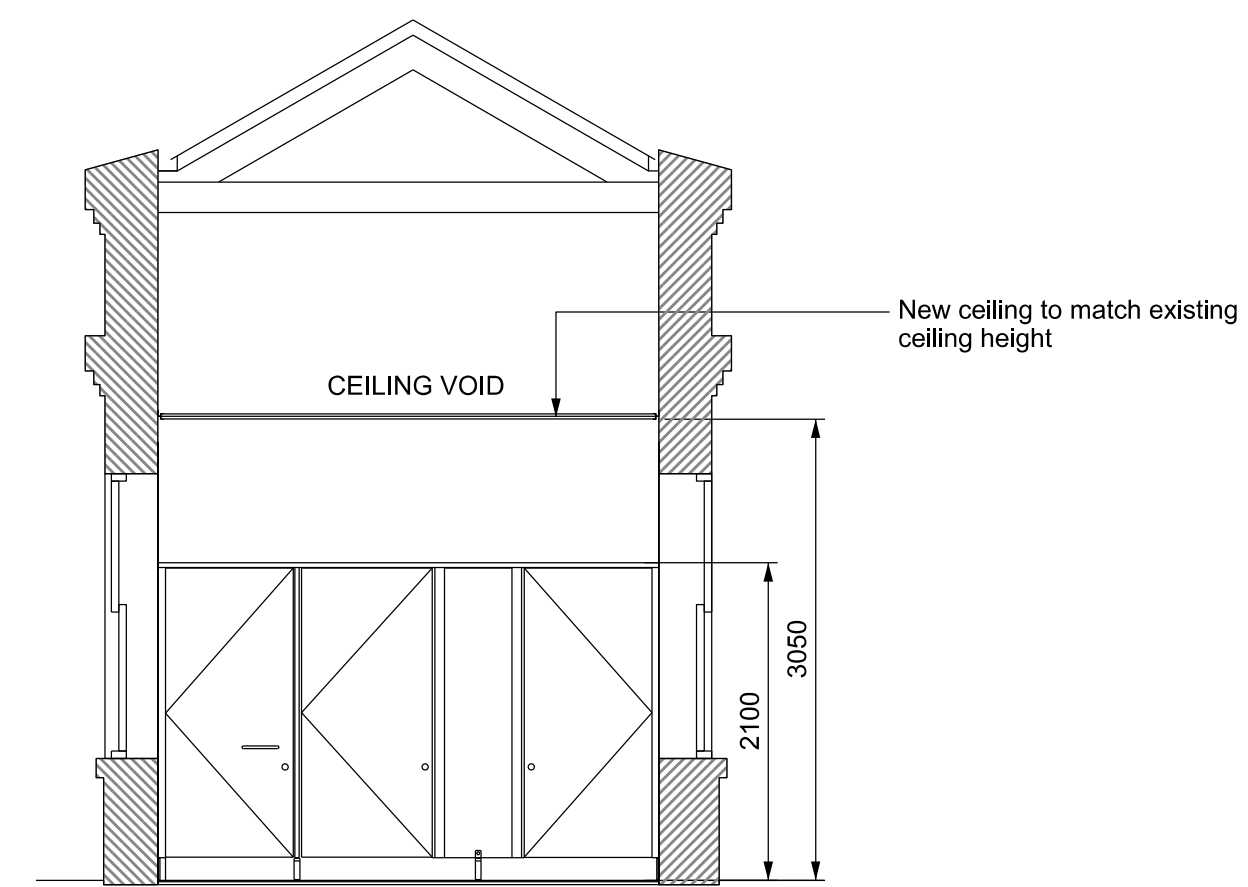
4 CROSSED SECTION 1:50
