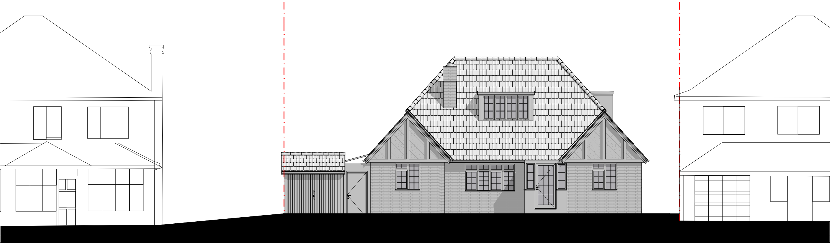
E-01 Extg Southeast (Front) 1:100
