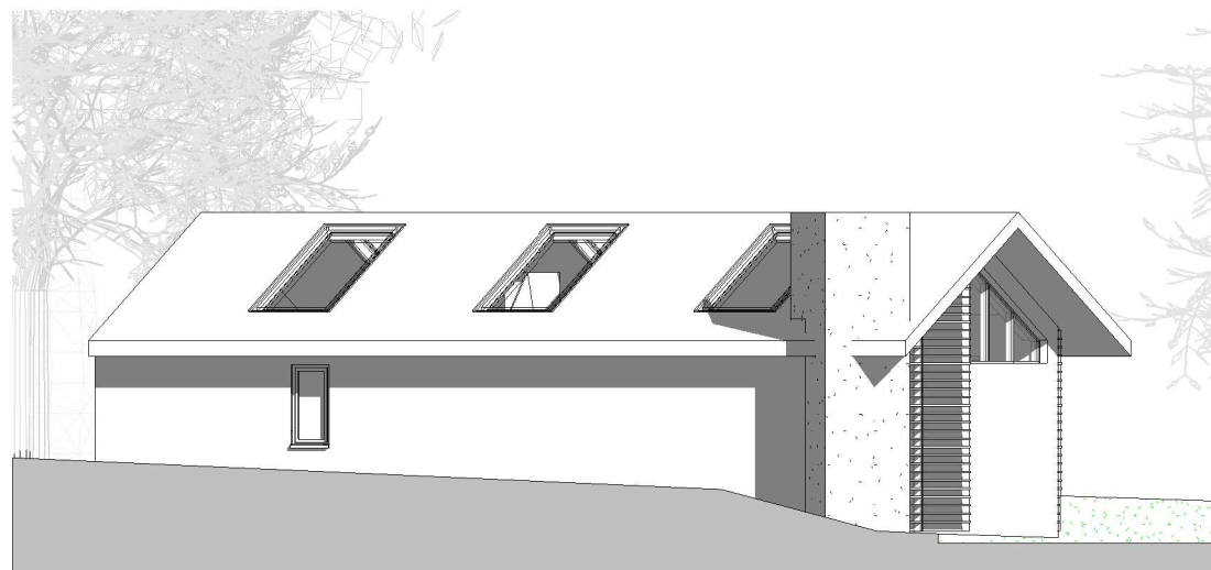
Proposed Side 1 Elevation 1 : 100
