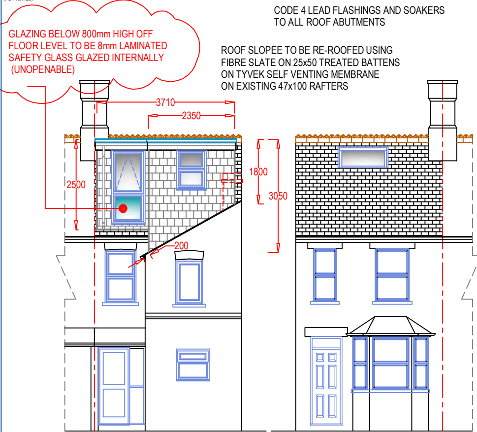
PROPOSED REAR ELEVATION (1:100) PROPOSED PRINCIPAL ELEVATION (1:100)
