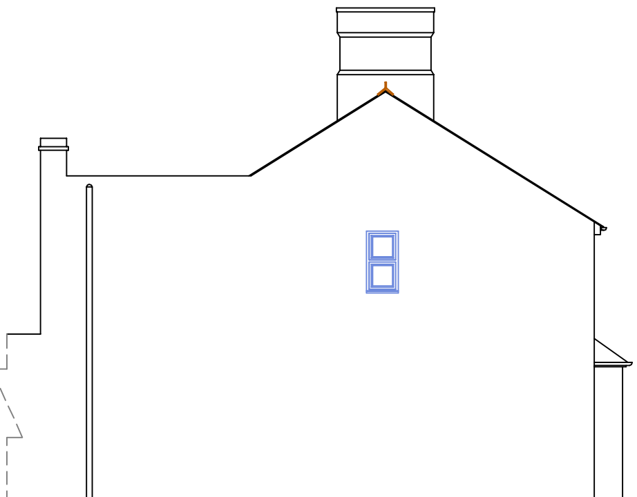
EXISTING SIDE ELEVATIONS (1:100)
