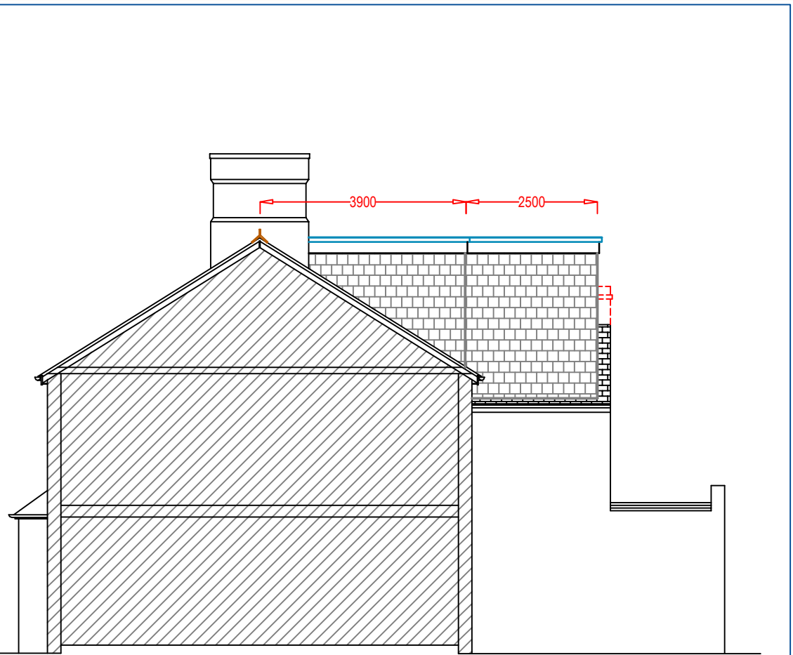
PROPOSED SIDE ELEVATIONS (1:100)
