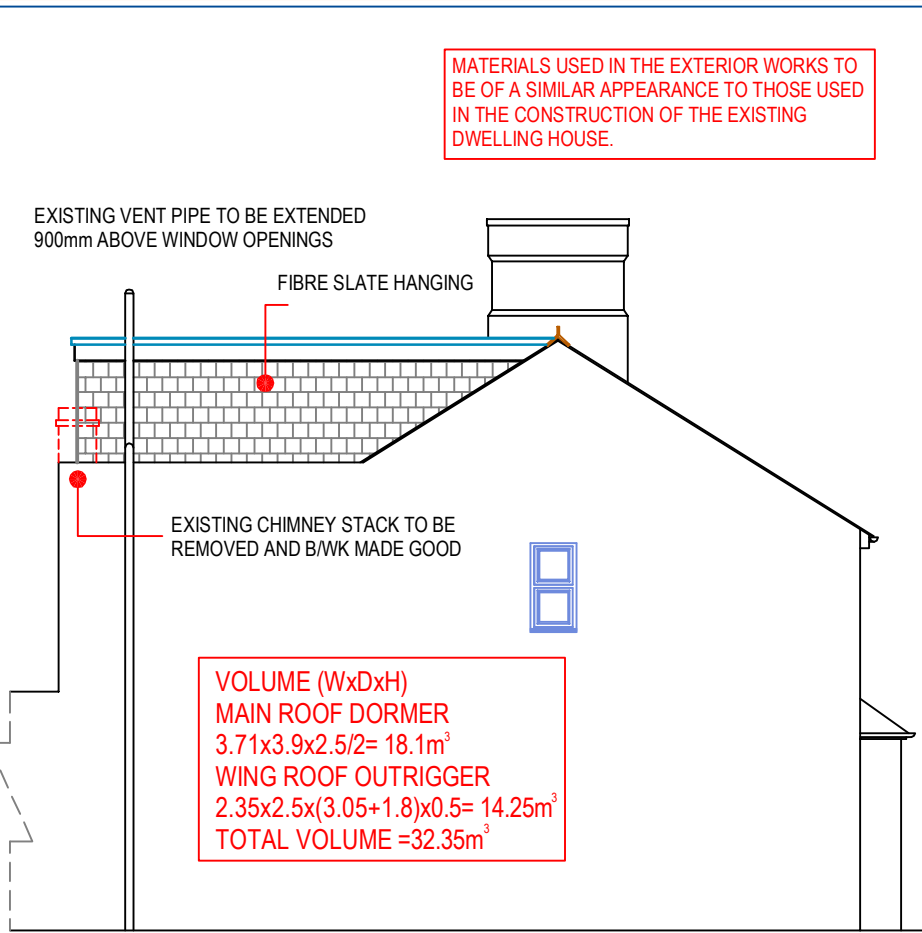
PROPOSED SIDE ELEVATIONS (1:100)
