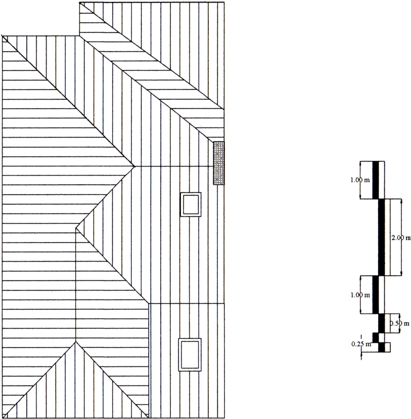
ROOF PLAN
