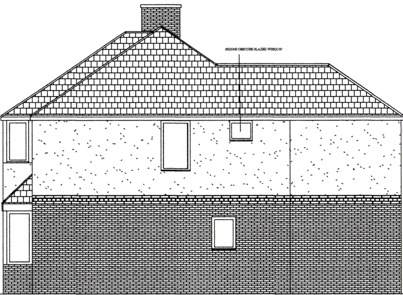
PROPOSED R/H ELEVATION
