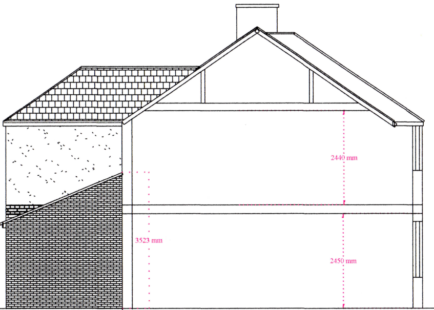
PROPOSED L/H ELEVATION
