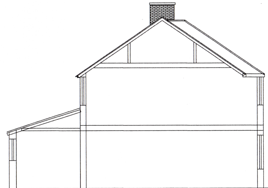
EXISTING L/H SIDE 1:100
