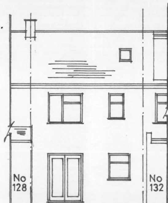
REAR ELEVATION 1:100 (existing)
