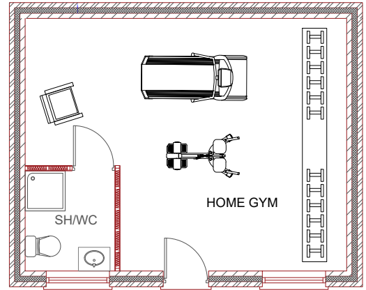
Proposed Ground Floor Scaled 1:100
