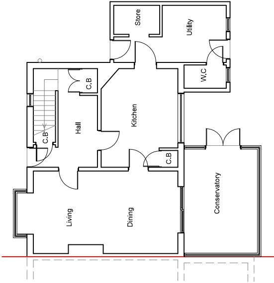
Existing Ground Floor Plan Scale 1:100
